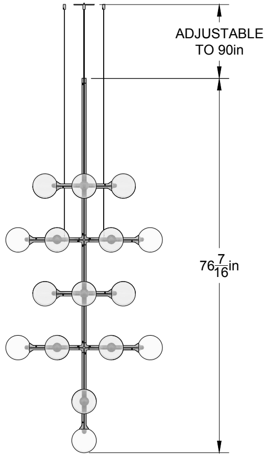
ELEVATION VIEW
