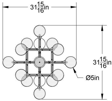
PLAN VIEW
