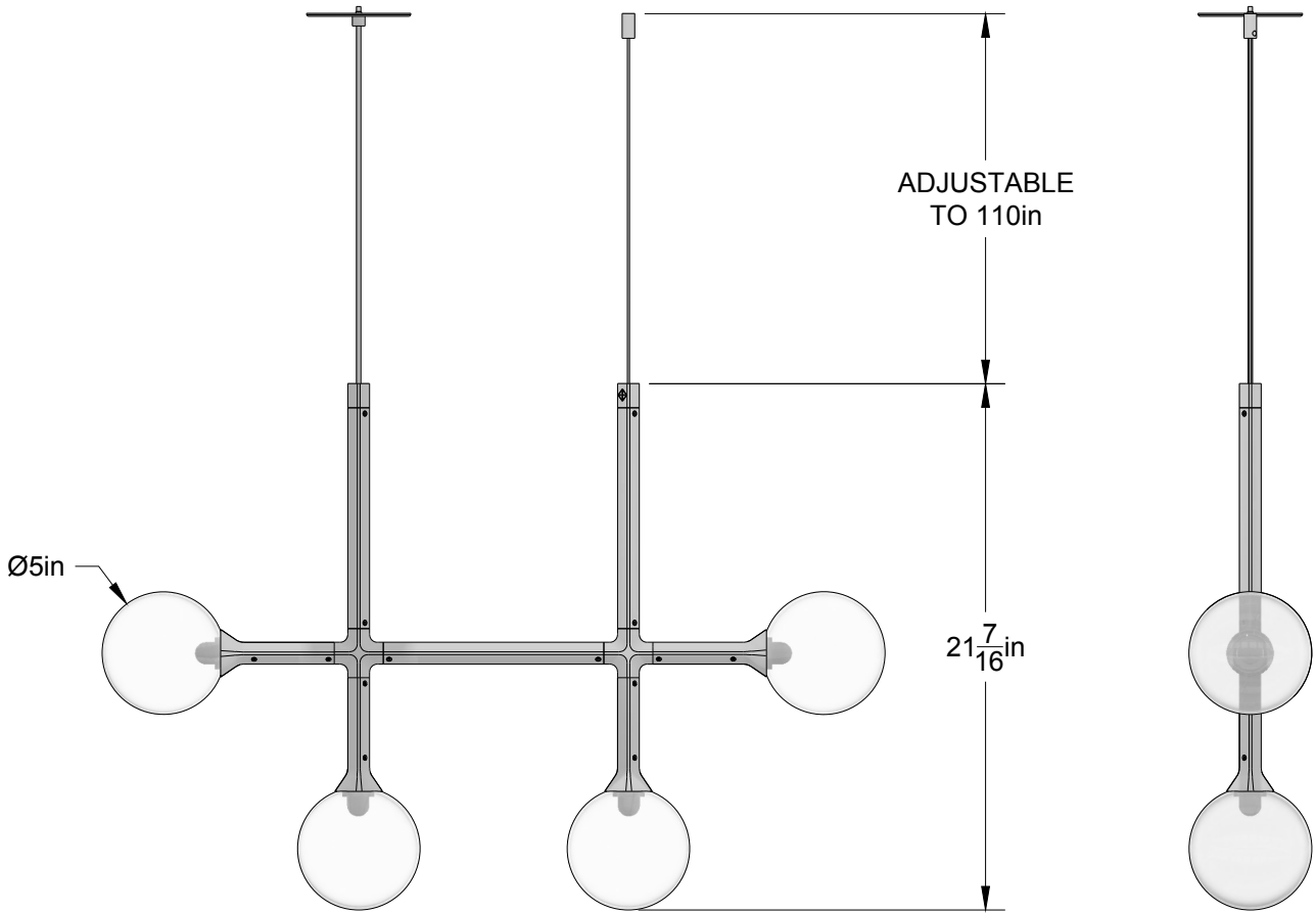
ELEVATION VIEW
