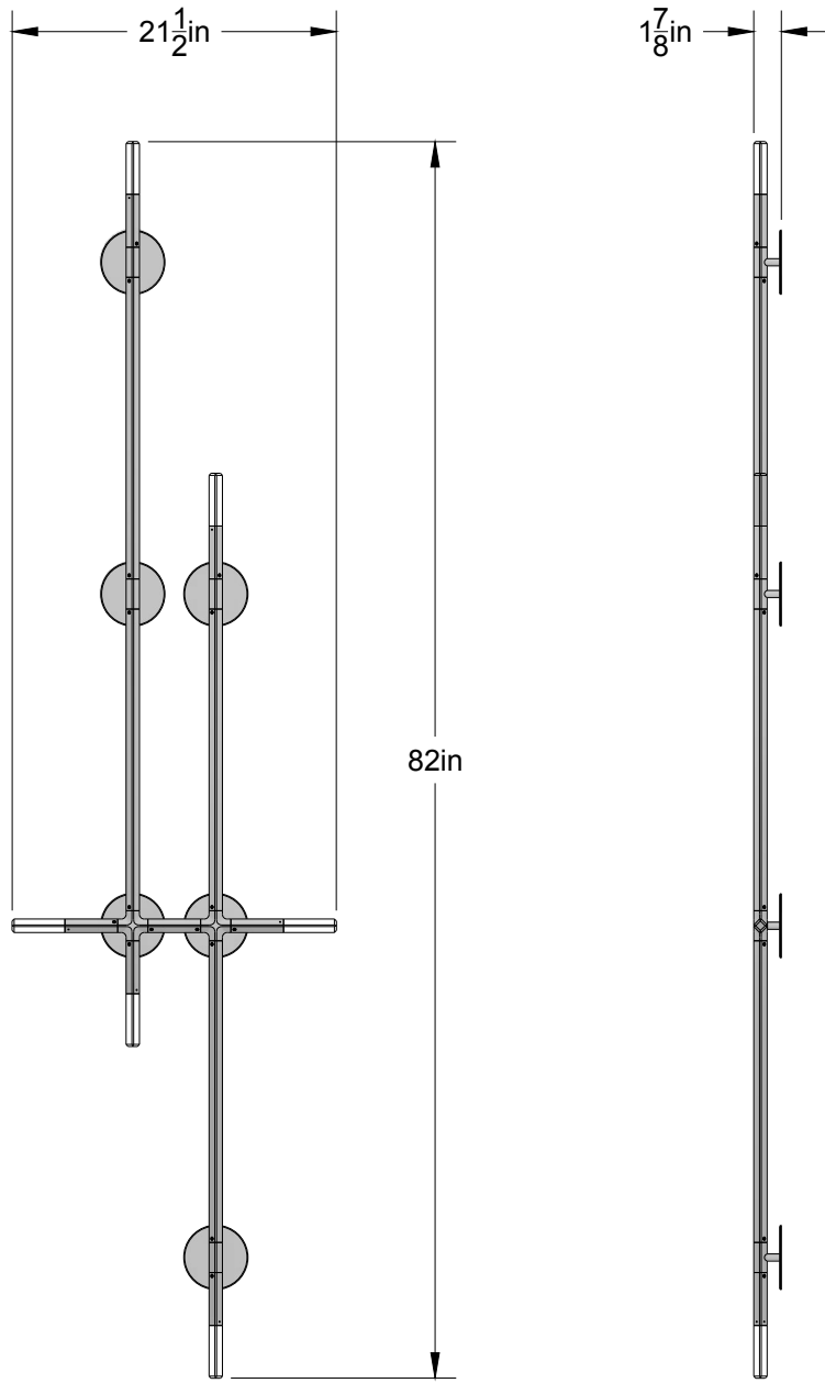
ELEVATION VIEW
