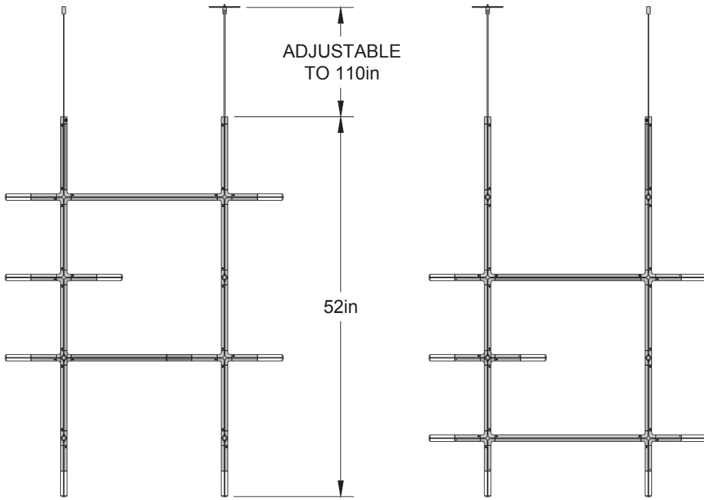
ELEVATION VIEW
