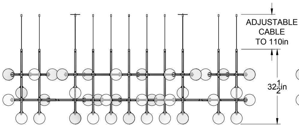
ELEVATION VIEW
