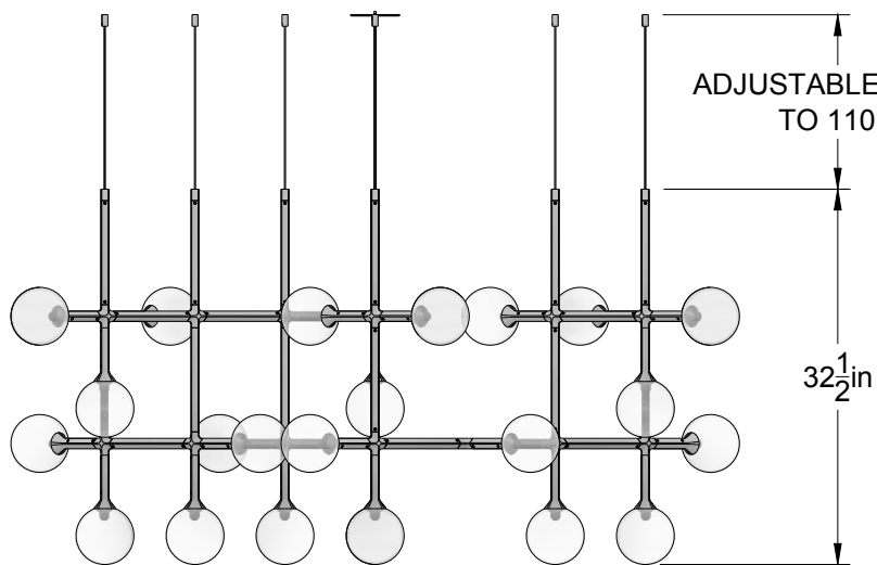
ELEVATION VIEW
