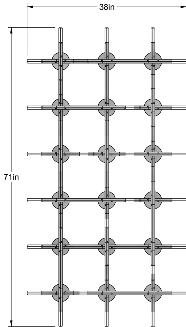
ELEVATION VIEW
